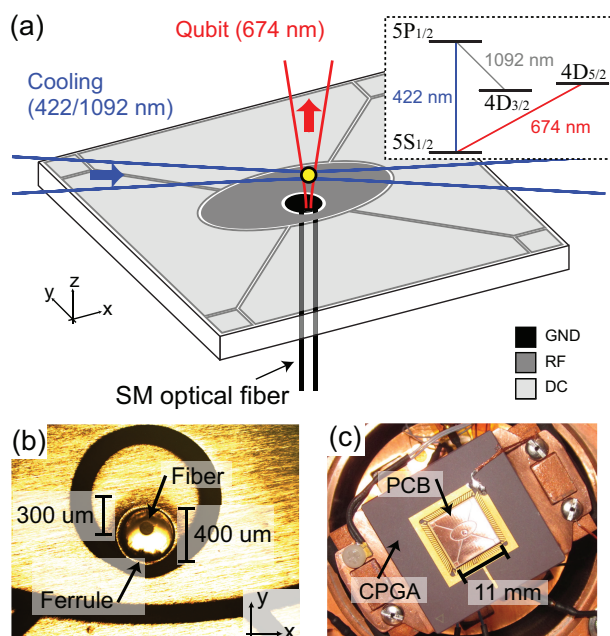
FIG. 1. (Color online) (a) Schematic of the surface-electrode ion trap with integrated optical fiber. The ^{88}\text{Sr}^+ qubit laser is delivered axially (along z ) through the fiber, while Doppler cooling beams propagate horizontally along \vec{e}_x - \vec{e}_y . (b) Alignment of the optical ferrule with respect to the trap electrodes. The ferrule is rotated until the fiber is aligned with the minor axis of the trap. (c) Fiber-trap system mounted on a CPGA and installed on the 8 K basplate of a closed-cycle cryostat.
