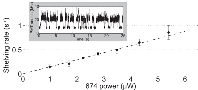
FIG. 2. Shelving rate as a function of 674 nm power coupled to the trap fiber. Inset: telegraph log of a single ion as it is shelved into the dark 4D_{5/2} state by 5.4 \mu\text{W} of fiber light.
