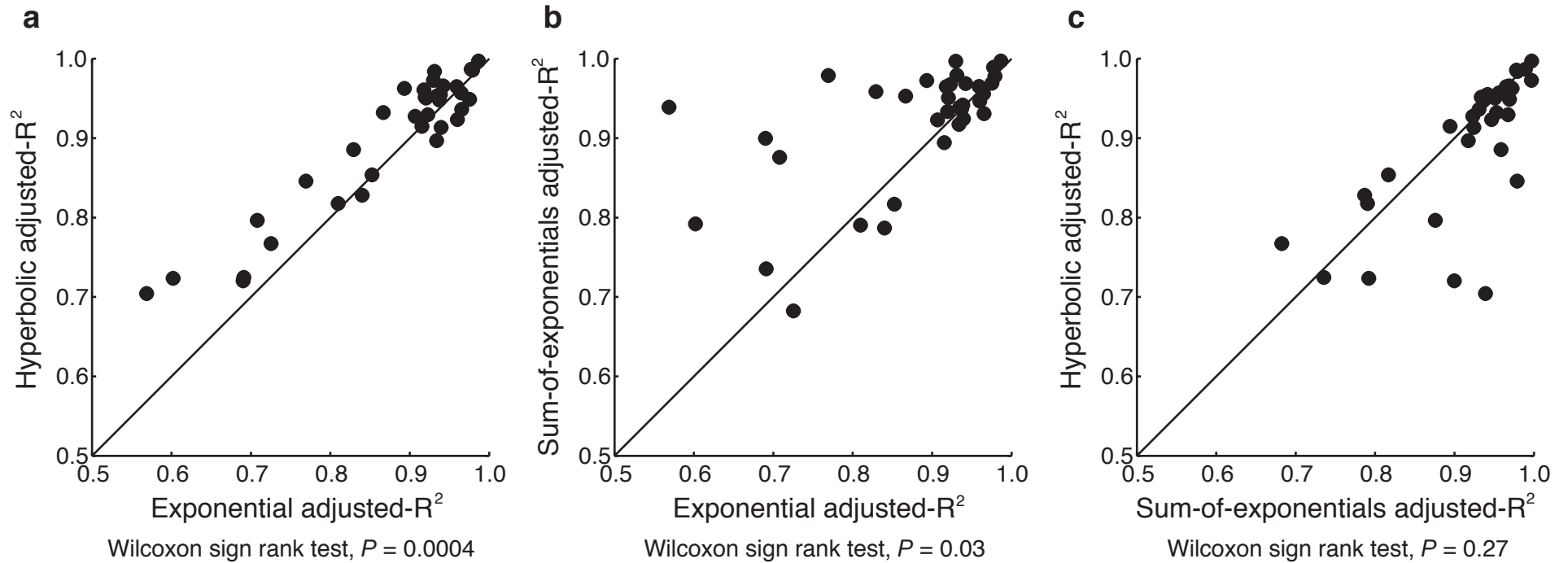
Supplementary Figure 2. Comparison of behavioral fits. (a) Plotted is the adjusted-R-squared for the one-parameter hyperbolic discount function versus the adjusted-R-squared for the one-parameter exponential discount function. Each point represents the fit from a single subject's data from a single paid session. (b) Plotted is the adjusted-R-squared for the two-parameter sum-of-exponentials discount function versus the adjusted-R-squared for the one-parameter exponential discount function. (c) Plotted is the adjusted-R-squared for the one-parameter hyperbolic discount function versus the adjusted-R-squared for the two-parameter sum-of-exponentials discount function.
