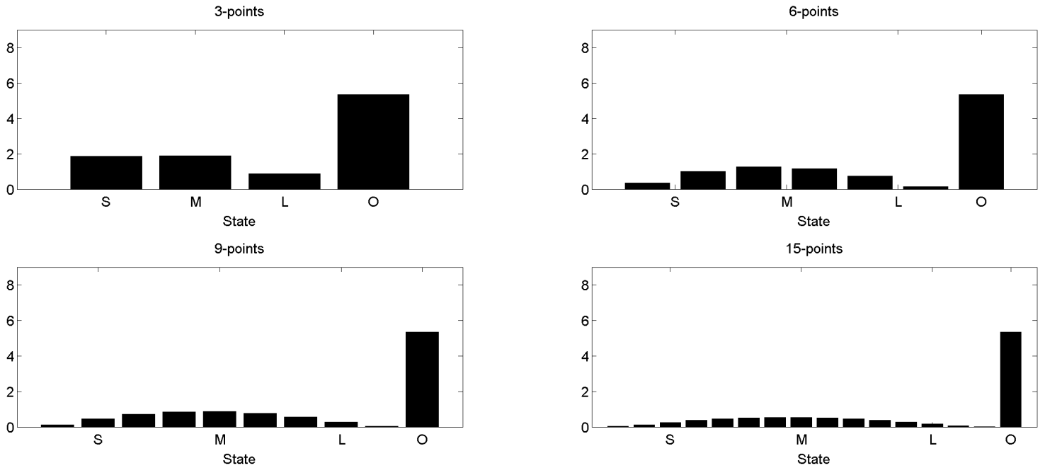
Figure 8: Firm size distribution as we change grid size, CW model
