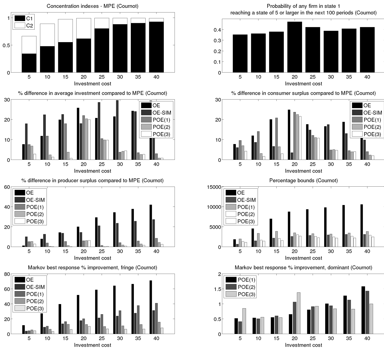
Figure 5: Long-run industry statistics for OE and POE versus MPE, Cournot model, \delta = 0.8
