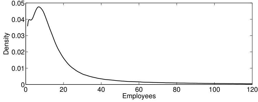
Figure D.1: Distribution of the number of employees
