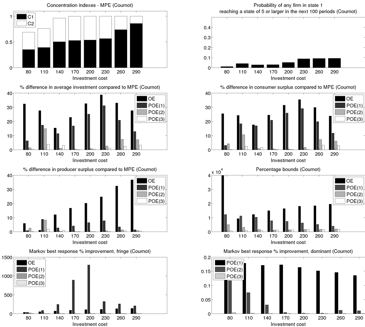
Figure 3: Long-run industry statistics for OE and POE versus MPE, Cournot model, \delta = 0.2
