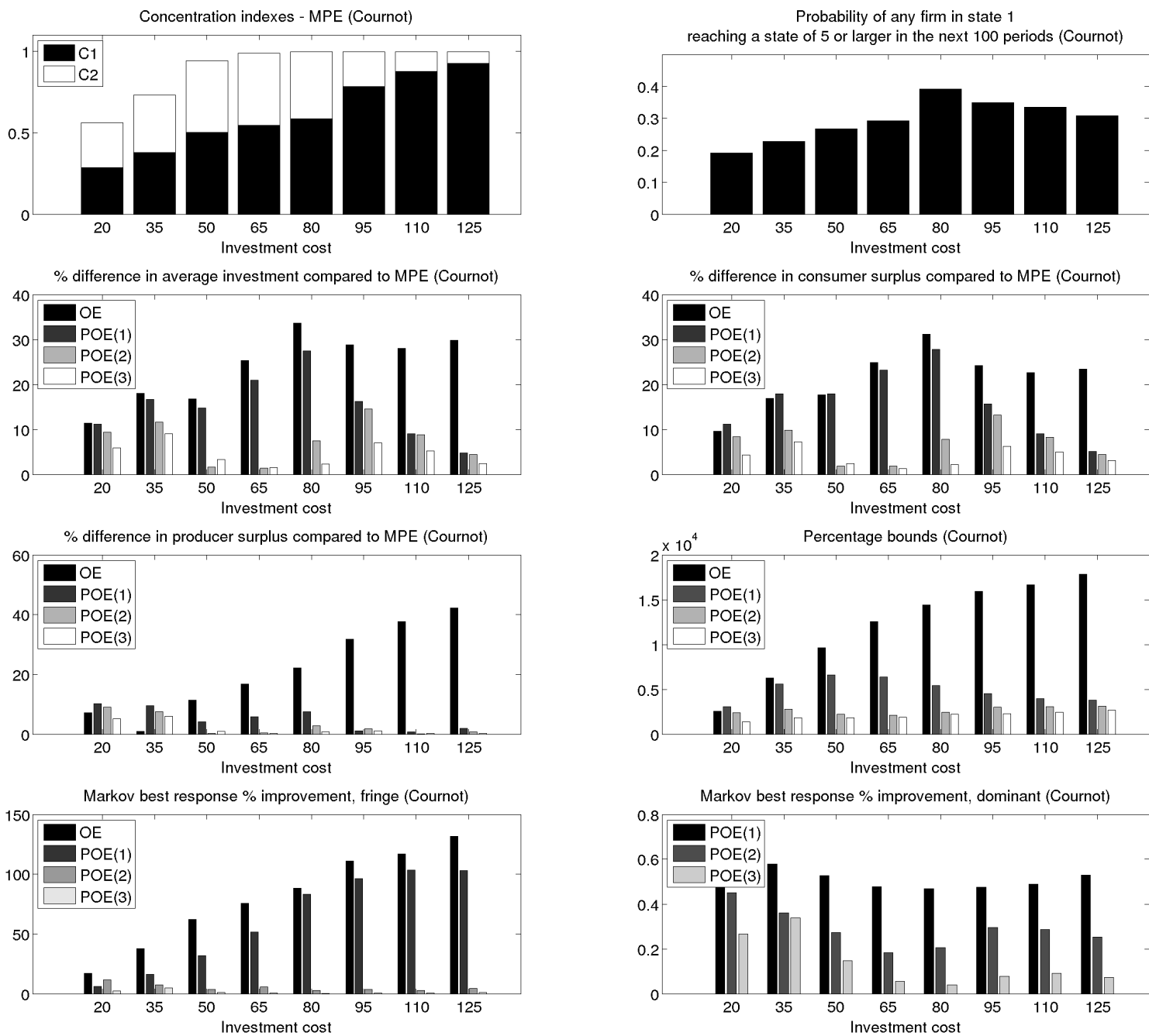
Figure 4: Long-run industry statistics for OE and POE versus MPE, Cournot model, \delta = 0.5
