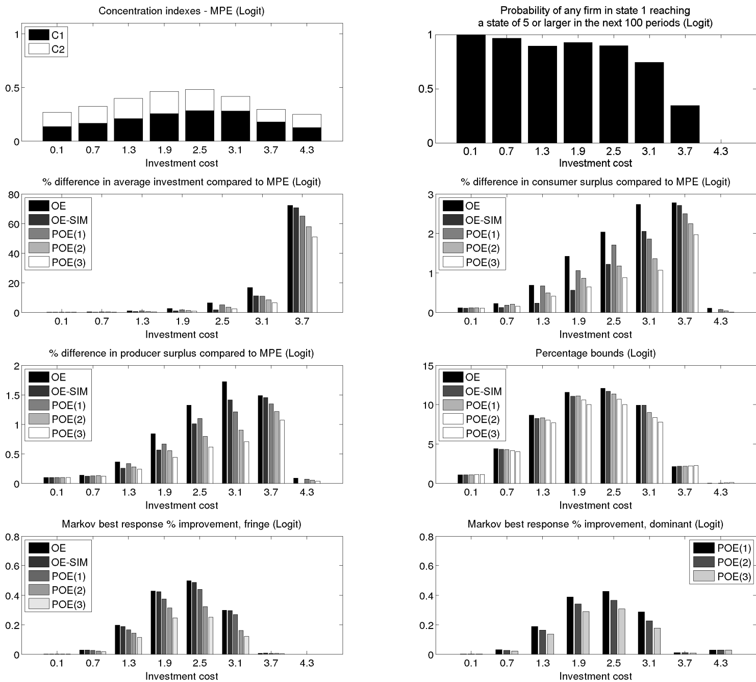
Figure 2: Long-run industry statistics for OE and POE versus MPE, logit model, \delta = 0.7
