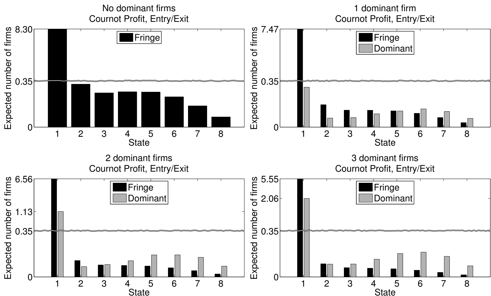
Figure 6: Long-run dominant/fringe state distribution, Cournot, investment cost=5
