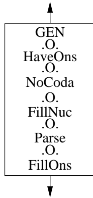
Figure 14: Lenient cascade
