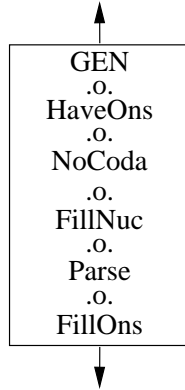
Figure 9: Merciless cascade.
