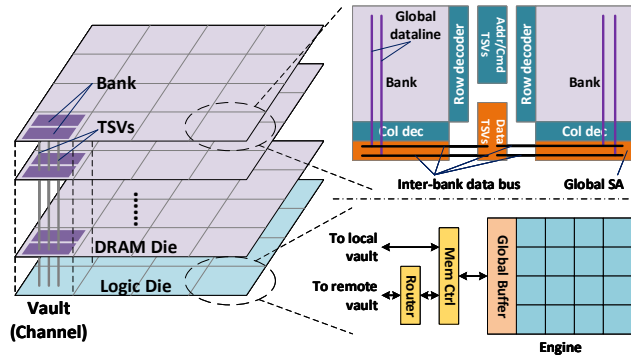
Figure 2. TETRIS architecture. Left: HMC stack. Right top: per-vault DRAM die structure. Right bottom: per-vault logic die structure.
