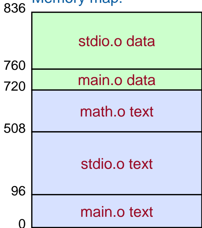
Memory map:
