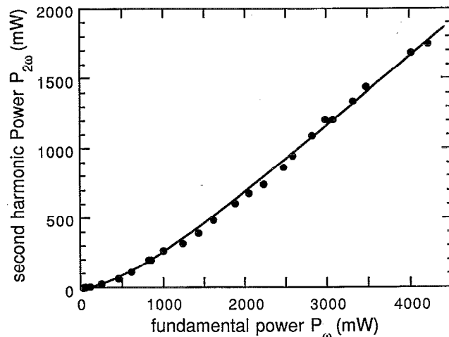
FIG. 2. Second harmonic power measured outside the cavity vs fundamental power incident on the cavity for a sample 1.24 mm in length with domain spacing of 3.47 \mu\text{m} . The sample was heated to 140^\circ\text{C} to achieve phase matching.
