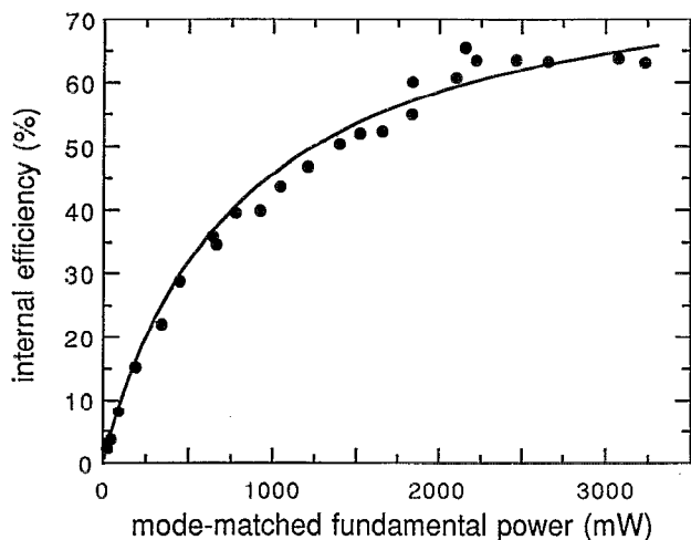
FIG. 4. Internal conversion efficiency for the periodically poled 1.24 mm sample.
