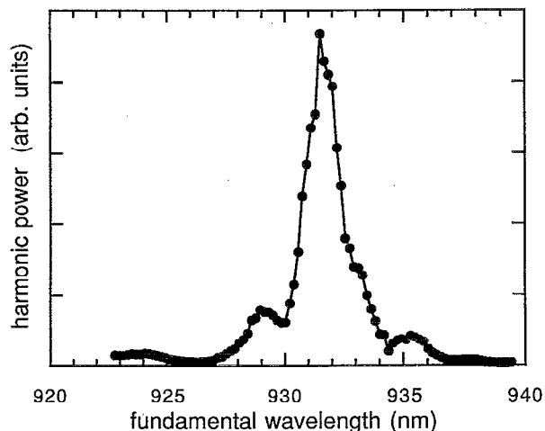
FIG. 1. Wavelength tuning curve for room-temperature single-pass SHG of a Ti:Al 2 O 3 laser in periodically poled LiNbO 3 .
