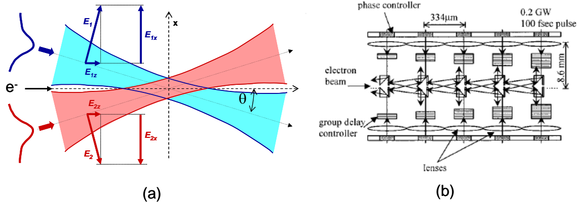
Figure 5: a) Electric field diagram for crossed laser beams. If the laser beams have opposite optical phases a nonzero longitudinal electric field remains but the transverse electric fields cancel. Optimum parameters for 1 micron wavelength lasers are beam spot sizes of about 30 microns, laser crossing angles of 15 mrad b) Originally proposed multistage accelerator structure employing crossed laser beams. High reflector surfaces and total internal reflection are used to guide the laser beams into the cascaded accelerator gaps each one having a length of \sim 1/3 mm [30].
