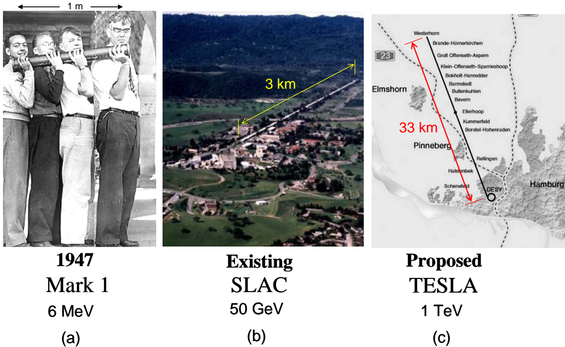
Figure 1: The growth of RF linear accelerators. a) The first 1 meter linear accelerator. It's inventor W.W. Hansen on the right. b) Aerial photograph of the Stanford Linear Accelerator center (SLAC) near Stanford University. c) Drawing of a proposed version of the 33 km TESLA accelerator in the vicinity of Hamburg as a possible candidate facility for the International Linear Collider (ILC)
