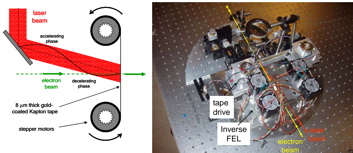
Figure 6: The successful version of the LEAP experiment. a) The laser-electron beam interaction on the slowly moving kapton tape. b) A photograph of the interaction region prior to incorporation into the vacuum system.
