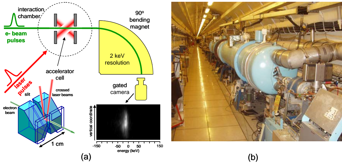
Figure 4: The LEAP experiment. a) Schematic diagram of the apparatus showing the accelerator cell, the energy spectrometer, and a real image of the typical observed electron beam spectrum, having a width of about 20 keV. b) View down the SCA accelerator. The blue cylinders in the foreground are the dewars containing the Niobium based superconducting accelerator. The LEAP experiment is located near the end of the tunnel.
