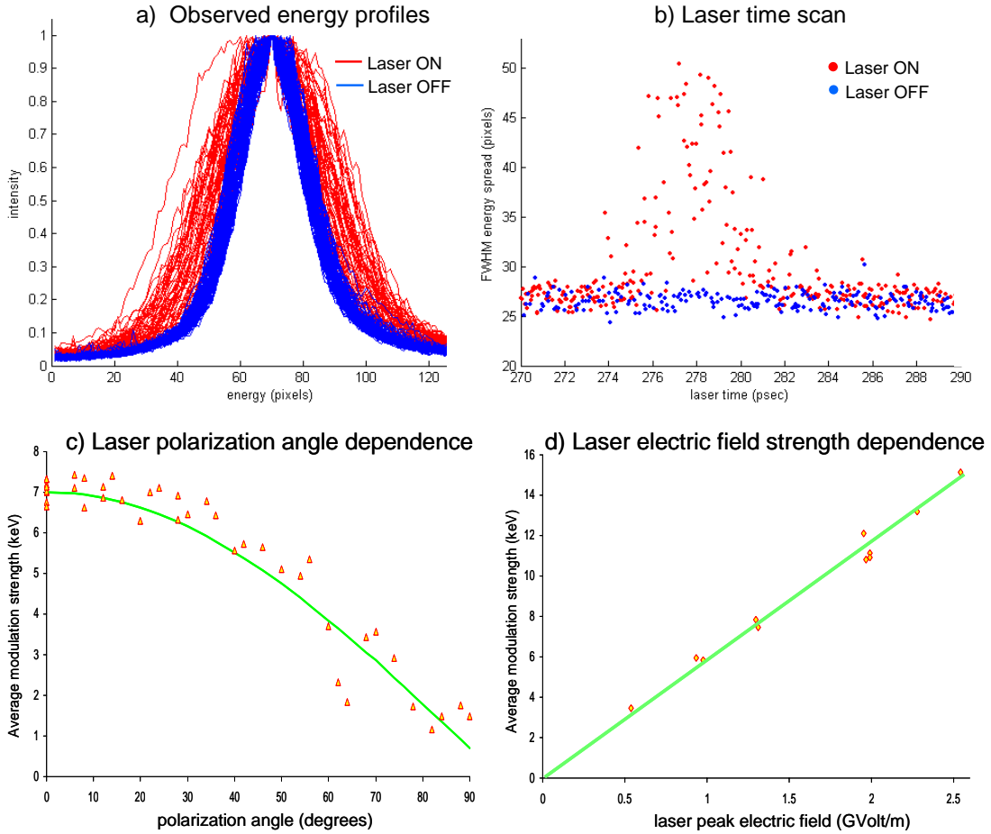
Figure 7: a) The energy spectra of multiple electron bunches. b) The FWHM of the energy spectra of the electron bunches as a function of laser delay time relative to the electron pulse. c) Dependence of the energy modulation strength on the laser polarization. d) Dependence of the energy modulation strength on the electric field strength of the laser
