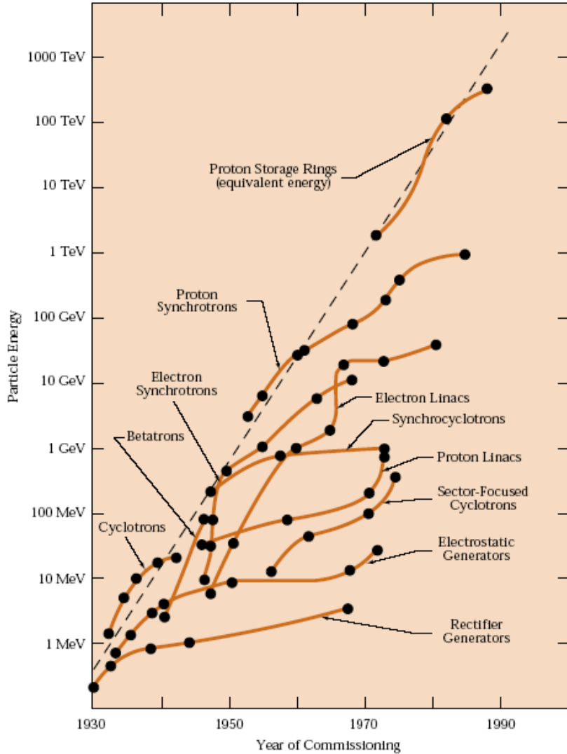
Figure 2: The Livingston Plot showing the exponential growth of particle beam energy versus year of commissioning.
