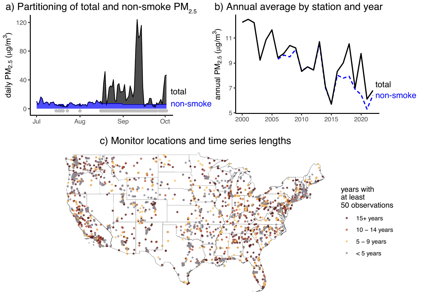
Extended Data Fig. 1 | Pollution stations and method used to construct non-smoke PM_{2.5} estimates. a. Example of total and non-smoke partitioning for a single station in CA in 2020. On days without a smoke plume overhead (no grey points), all PM_{2.5} is assumed to be from non-smoke sources. On days with a plume overhead (grey points), PM_{2.5} anomalies from the non-smoke month- and station-specific 3-year median are attributed to smoke, and total
