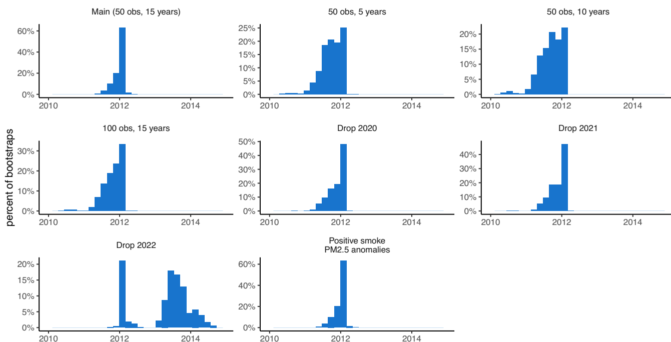
Extended Data Fig. 2 | Distribution in estimated breakpoints for different sample restrictions and/or statistical specifications. a. Annual average PM 2.5 . b. Extreme (> 35 µg/m 3 ) daily PM 2.5 . Histograms show distribution of estimated breakpoints for different sample restrictions, pooling data from all CONUS monitors. Panels labeled with number of observations and years are various sample restriction choices, while those labeled “Drop” retain our primary inclusion criteria – more than 50 observations per year for at least 15
