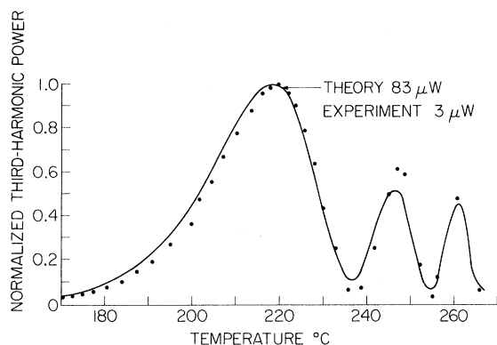
FIG. 1. Normalized third-harmonic power versus temperature for pure Rb vapor. The 50-kW 1.064- \mu m beam was focused on the output cell window with a confocal parameter of 40 cm.
