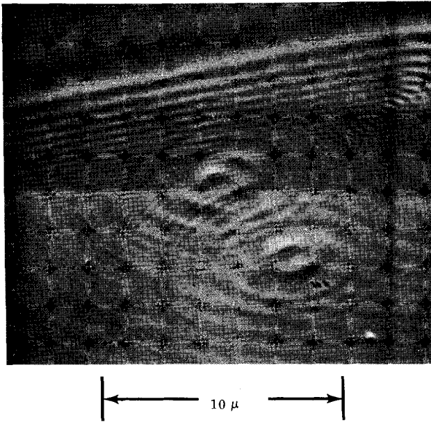
FIG. 2. SEM picture of holograms of 1.305- \mu -diam particles. (25-kV electron potential, 60° sample tilt.)
