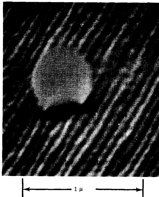
FIG. 1. SEM picture of 836-Å spaced fringes produced in PMMA by 1182-Å radiation. The round object is a 0.500-μm-diam latex sphere placed on the fringes after development for magnification calibration. (25 kV electron potential, 80° sample tilt.)
