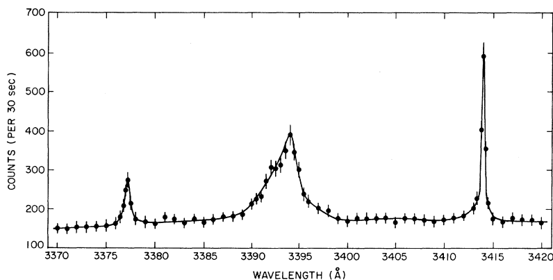
FIG. 2. Magnitude of the spontaneous radiative emission at 3394 Å with 10 Torr of argon buffer gas. Two tabulated Ba transitions at 3377.4 and 3413.8 Å serve as a convenient wavelength calibration and illustrate the characteristic difference between the line shape of a radiative collisional emission and the fluorescence from a real line. The scan has not been corrected for the 0.5-Å ( \sim 4\text{-cm}^{-1} ) spectrometer resolution.
