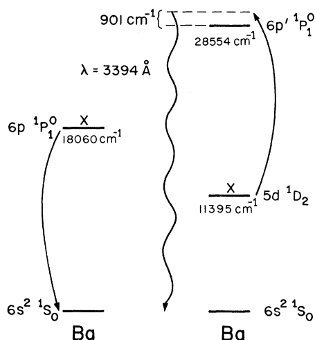
FIG. 1. Pertinent Ba levels for observation of radiative collisional fluorescence. A Ba atom in the 6p\ ^1P_1^{\circ} state collides with a Ba atom in the 5d\ ^1D_2 state, causing the emission of a photon at the sum energy (3394 Å) and the simultaneous deexcitation of both atoms.
