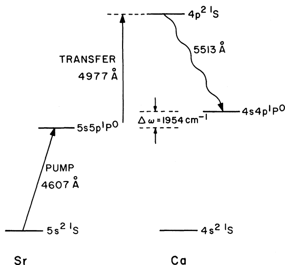
FIG. 1. Energy level diagram for Sr* + Ca + \hbar\omega \rightarrow Sr + Ca* switched collision process.
