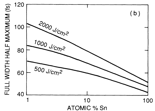
FIG. 3. (a) X-ray peak power conversion efficiency ( \lambda = 3.6 Å) as a function of percent tin. (b) X-ray pulse width for a 100-fs laser pulse.
