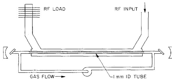
Fig. 3. Schematic of the small volume, direct coupled, microwave-pumped cell.
