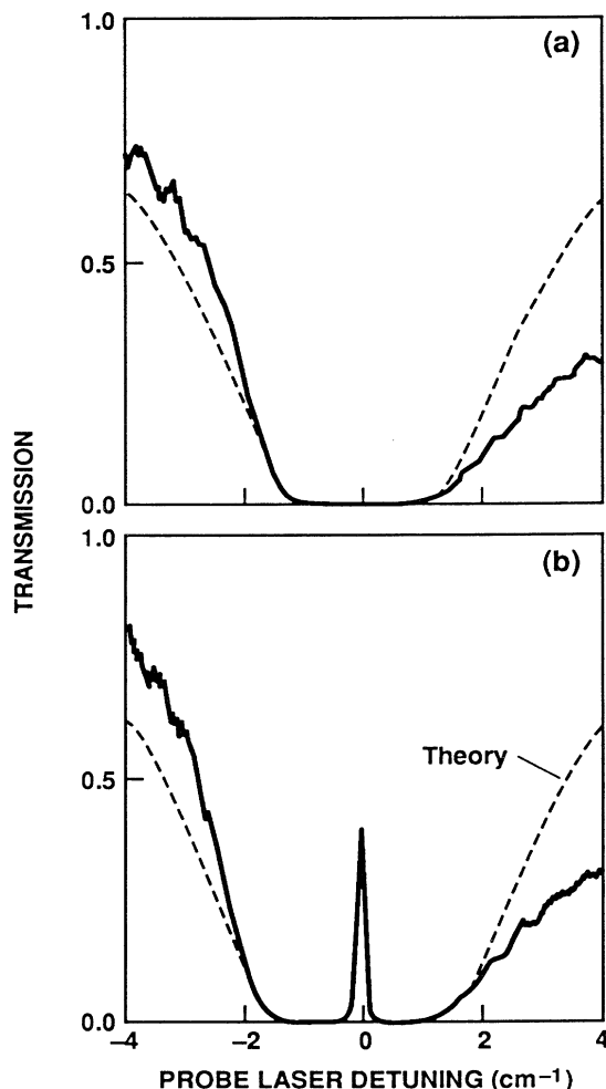
FIG. 3. Transmission vs probe laser detuning for (a) \Omega_{23}=0 and (b) \Omega_{23}=1.5 \text{ cm}^{-1} , \Delta\omega_c = -0.1 \text{ cm}^{-1} . Minimum transmission is \exp(-20) .
