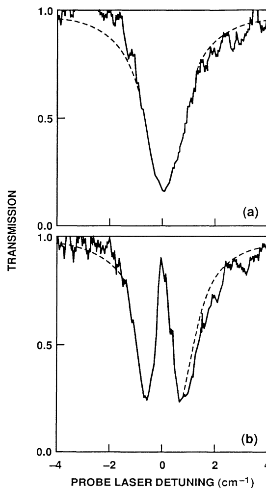
FIG. 2. Transmission vs probe laser detuning for (a) \Omega_{23}=0 and (b) \Omega_{23}=1.3 cm -1 , \Delta\omega_c=-0.2 cm -1 . Minimum transmission is \exp(-1.7) .
