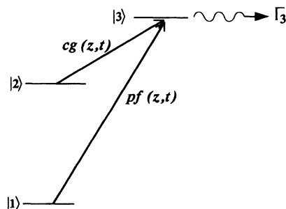
FIG. 1. Energy level diagram. States |1\rangle - |2\rangle are stable; state |3\rangle decays to other states which are not shown. Electromagnetic pulses pf(z,t) and cg(z,t) are applied on the |1\rangle - |3\rangle and |2\rangle - |3\rangle transitions.
