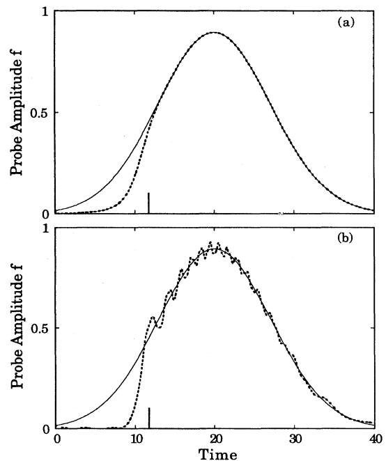
FIG. 4. Probe amplitude vs local time (s) at z=0 (solid lines) and z=50 (dashed lines). \Omega_p = \Omega_c = 10 . All other conditions are the same as in Fig. 2.
