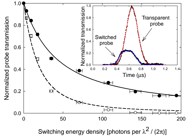
FIG. 5. (Color online) Probe transmission [raw data (●) and data corrected for Gaussian spatial profile (○)] is normalized to EIT transmission of 60%. All lasers are on resonance, \Omega_c^{(1)}=\Omega_c^{(2)}=2.0\Gamma_3 , \Omega_c^{(3)}=1.7\Gamma_3 , N\sigma_{13}L=7.5 , and \gamma_{12}=0.15\Gamma_3 . Inset: Probe pulse (raw data) with and without the switching laser applied.
