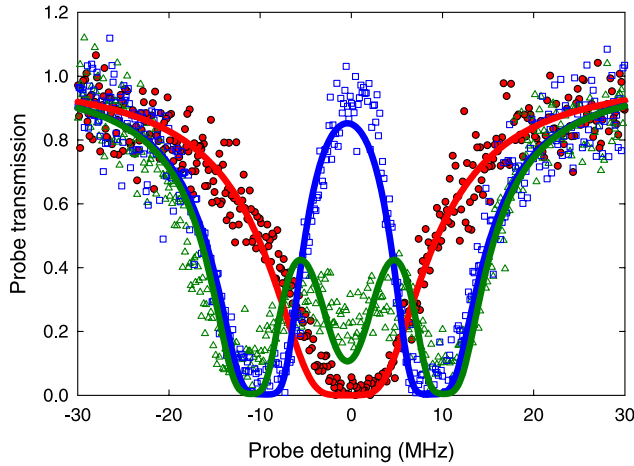
FIG. 4. (Color online) Probe transmission for absorption (●), EIT (□), and switching (△) averaged over ten atom clouds. Data are taken by detuning the probe laser while switching and coupling lasers are on resonance. The solid lines represent a simultaneous, least-squares fit to all three curves where N\sigma_{13}L=8.9 , \gamma_{12}=0.1\Gamma_3 , \Omega_c^{(1)}=\Omega_c^{(2)}=3.6\Gamma_3 , \Omega_c^{(3)}=2.9\Gamma_3 , \Omega_s^{(1)}=1.1\Gamma_3 , \Omega_s^{(2)}=1.5\Gamma_3 , and \Omega_s^{(3)}=2.0\Gamma_3 .
