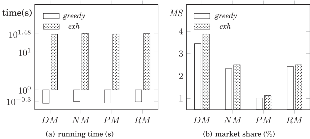
Fig. 2. Varying distance metrics: greedy vs. exh .
