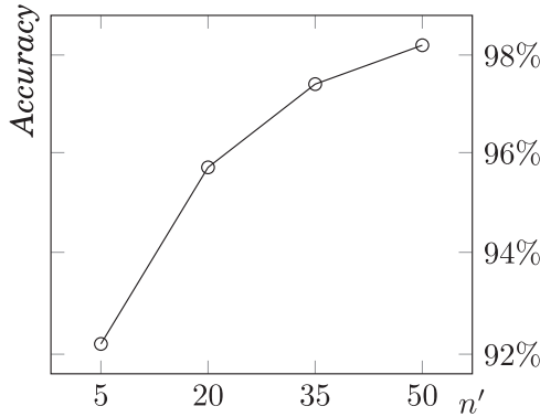
Fig. 9. Accuracy of learning from arbitrary guess.
