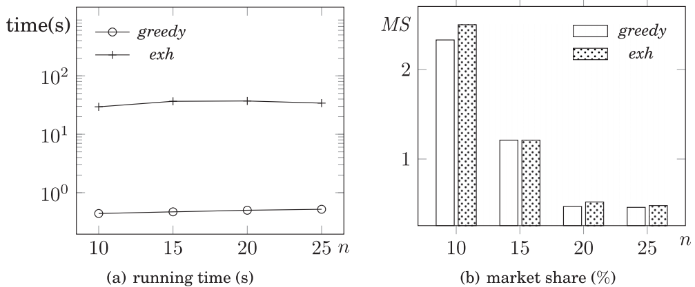
Fig. 5. Varying d : greedy vs. exh .
