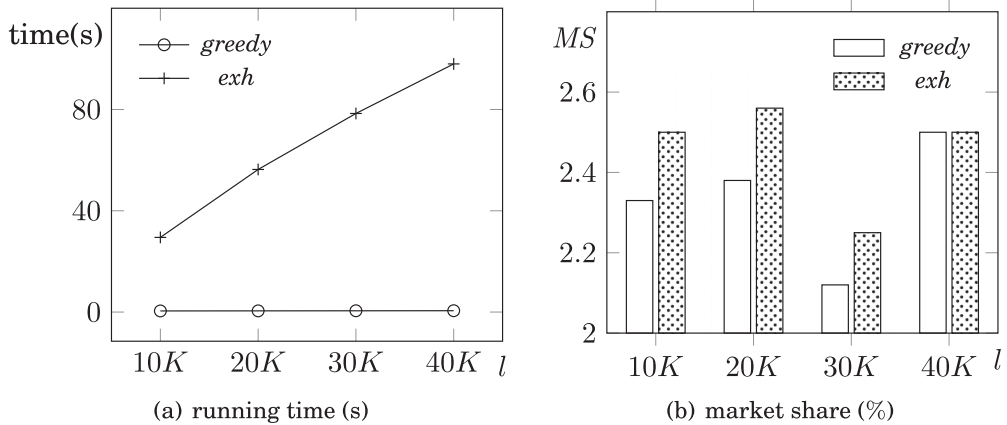
Fig. 3. Varying l : greedy vs. exh .
