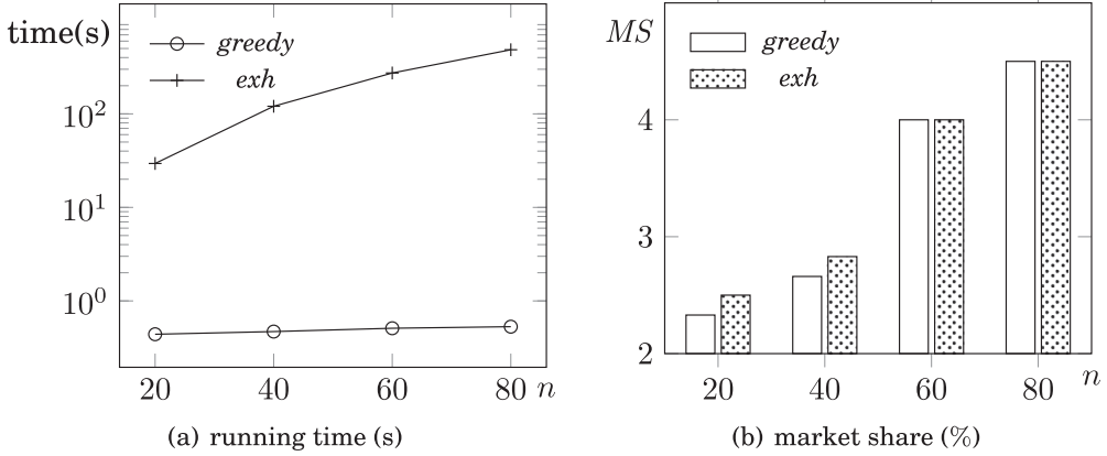
Fig. 6. Varying n : greedy vs. exh .
