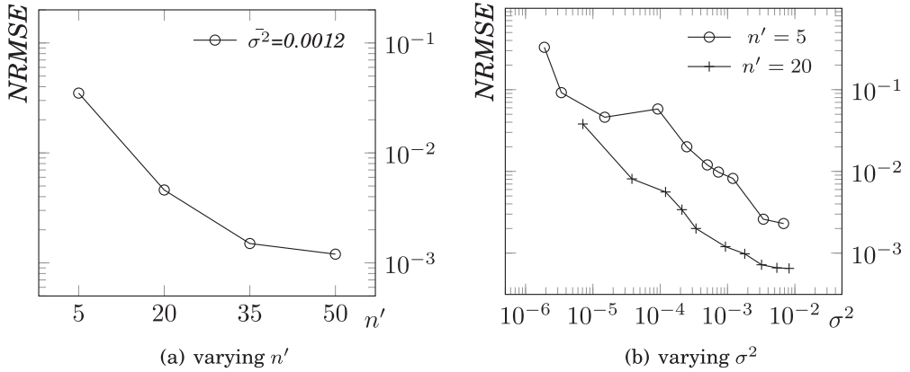
Fig. 8. Accuracy of learning from perfect knowledge.
