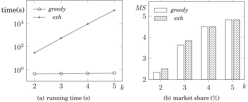
Fig. 7. Varying k : greedy vs. exh .
