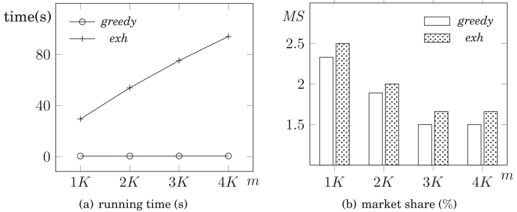
Fig. 4. Varying m : greedy vs. exh .
