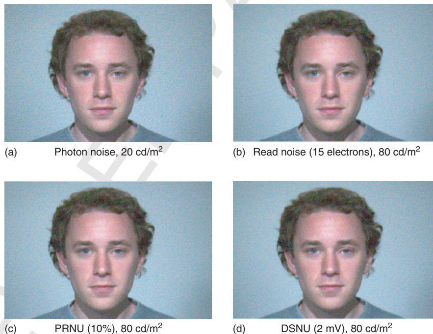
Figure 9 Sources of noise. Processed images from a sensor with the Bayer CFA, 1.7 micron pixel and 15 ms exposure duration. Photon noise is visible when the mean scene luminance is 20 cd/m 2 (a). Image noise due to read noise (b), PRNU (c), and DSNU (d) when the scene luminance is 80 cd/m 2 is also visible.
