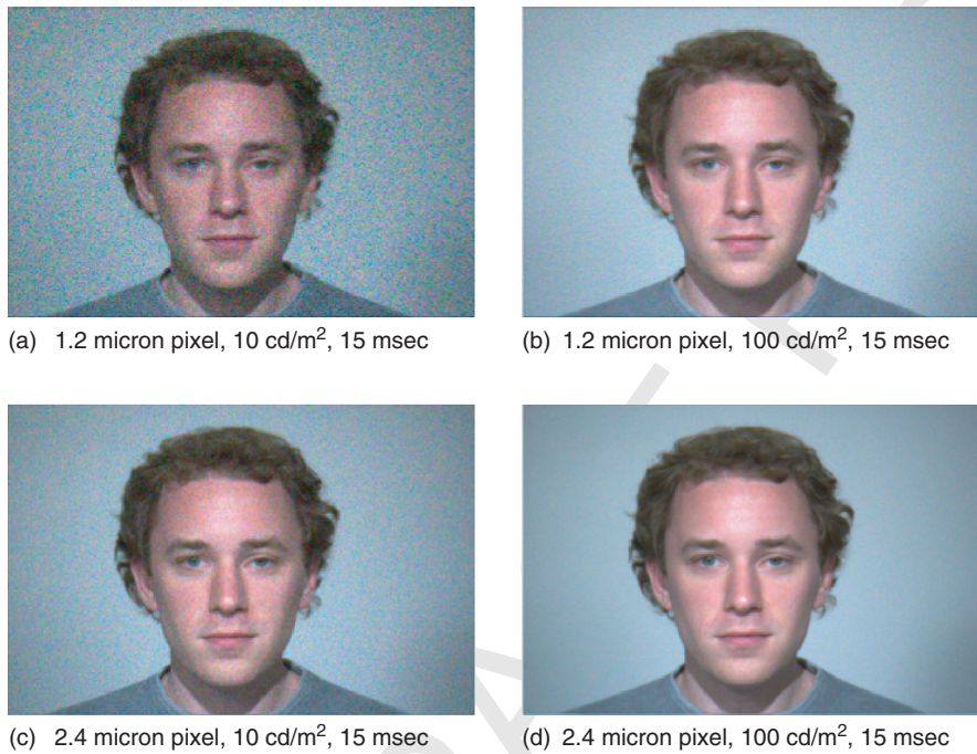
Figure 10 Photon noise. The processed images shown at (a,b) were calculated using a simulated imaging sensor that has a 1.2-micron pixel and a 15-ms exposure duration. (c,d) were calculated using a simulated imaging sensor that has a 2.4-micron pixel and a 15-ms exposure
