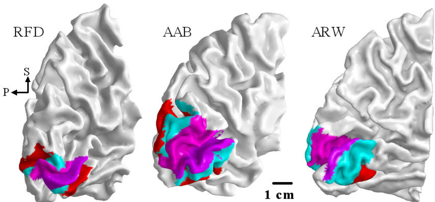
Figure 6. Position and size of the 2-12 degree region of V1, V2 and V3 in three hemispheres. The color convention is the same as in Figure 5: V1 is indicated by magenta, V2 by cyan and V3 by red.
