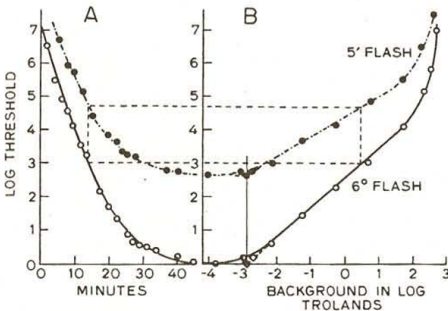
FIG. 34. Panel A: recovery curves for 5' (top) and 6° (bottom) test lights following offset of 3,600' conditioning field. Panel B: increment-threshold curves for the same test lights superimposed on a 3,600' steady-background field. [From Blakemore and Rushton (22).]
