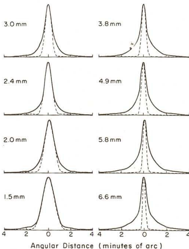
FIG. 7. Pointspread functions of the human eye for white light at various pupil diameters. Solid curves , radial profiles of theoretical pointspread functions calculated from linespread curves in Fig. 6. Narrower dashed curves , the point spread resulting from diffraction alone. [From Gubisch (59).]
