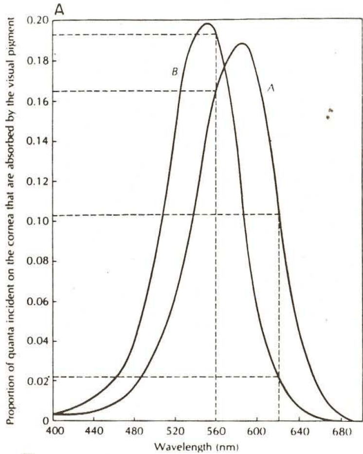
FIG. 23. A : absorption spectra for two classes of cones. (These are two of the three classes present in the normal human eye.) B : two-dimensional visual action space of a person whose eyes contain only the two kinds of cones plotted in A . See text for derivation of system B from A . [From Cornsweet (36).]
