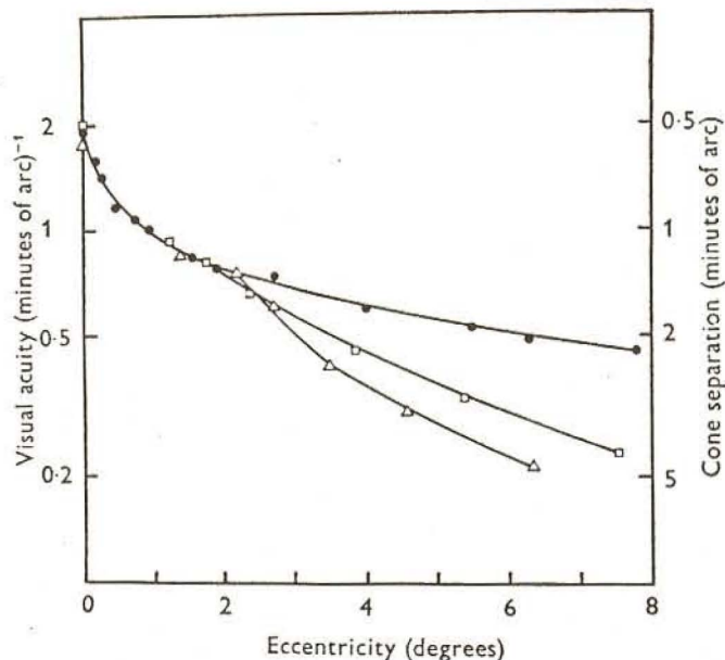
FIG. 16. Comparison between local spatial acuity for interference targets (633 nm) and intercone spacing at various distances from the center of the fovea ( 0^\circ eccentricity). Closed circles show center-to-center intercone distances (1/distance in min). Open points show local spatial acuity for two observers. Visual acuity here is arbitrarily defined as twice the highest resolvable spatial frequency in cycles/min. This definition allows a direct comparison between local spatial acuity and local cone density: if acuity and cone density were matched according to the sampling theorem, both should fall on a common curve—as they do out to 2^\circ . Targets subtended 32.4 min; mean intensity level was 1,200 trolands. [From Green (58), with permission from Cambridge University Press.]
