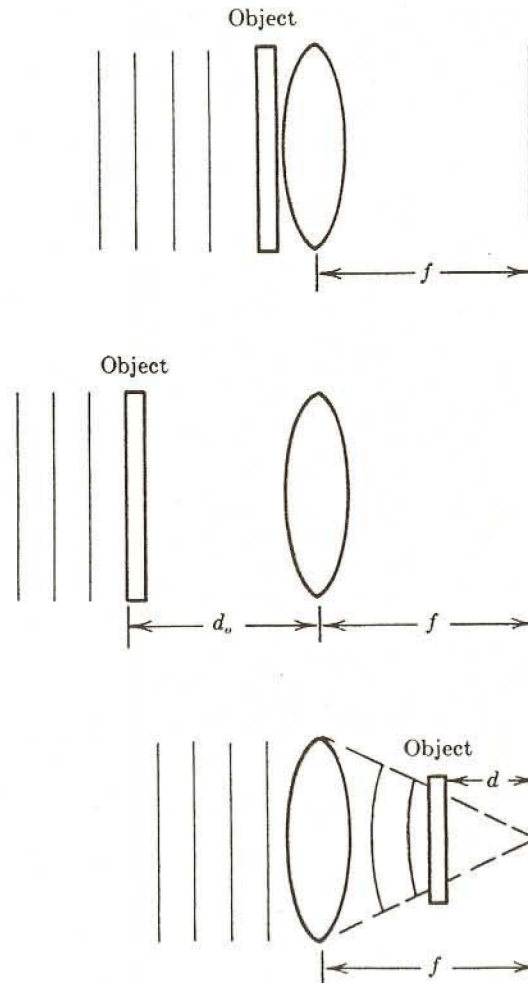
FIG. A5. Configurations for producing optical Fourier transforms. The focal length of the lens is represented by f ; thin vertical lines represent the illumination (a monochromatic plane wave). [From Goodman (51).]
