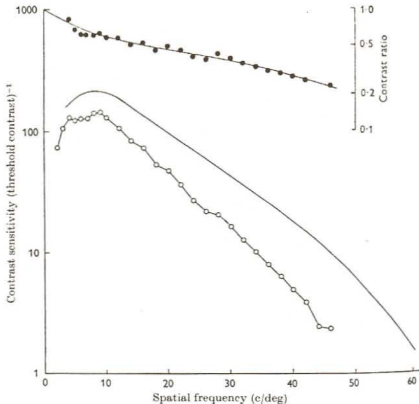
FIG. 15. Spatial contrast-sensitivity functions for interference fringes and normal targets at same mean retinal illuminance (500 trolands). Continuous smooth curve in lower portion of figure taken from data (closed circles) of Fig. 14 (i.e., these are interference target thresholds). Open circles show contrast thresholds for targets viewed normally, i.e., through the optics of the eye. Closed circles in the top portion show the ratio between the two curves below: this is an inferred measure of the modulation transfer function of the optics of this observer's eye. [From Campbell and Green (32), with permission from Cambridge University Press.]
