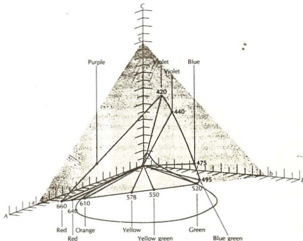
FIG. 29. A plane through trichromatic action space, showing the hue names of some of the stimuli it represents. The slightly curved triangular line in the shaded plane is the locus of the intersections of lights of all wavelengths with the plane. Therefore, it encloses a space representing the effects of all possible mixtures of wavelengths. [From Cornsweet (36).]
