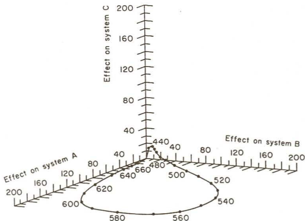
FIG. 28. Representation of the three-dimensional action space of the normal human visual system. The curved figure is the locus of the effect of the three systems of all wavelengths at a fixed intensity. [From Cornsweet (36).]
