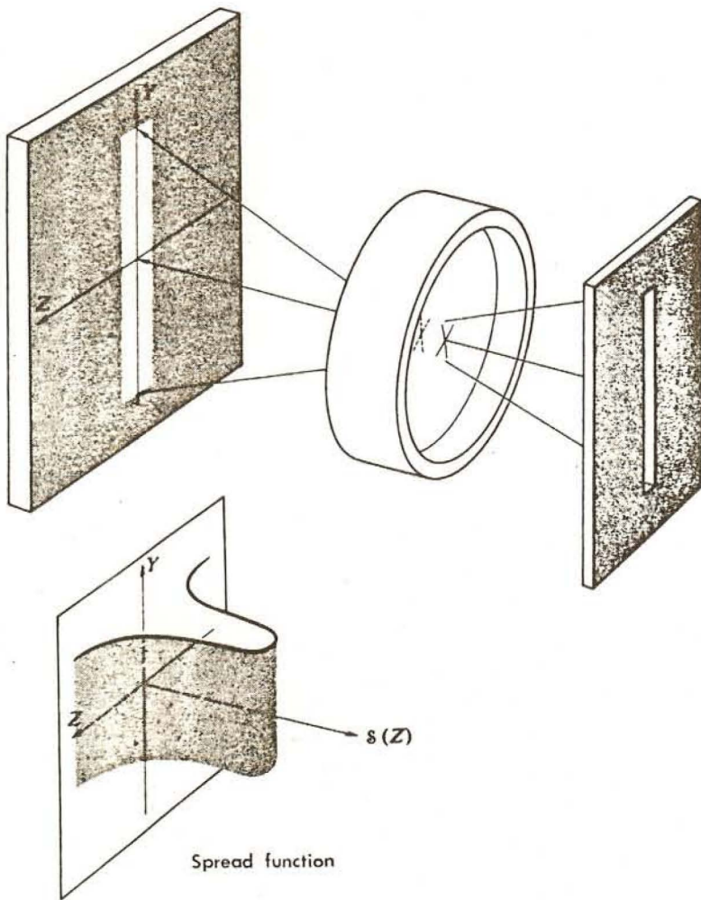
FIG. 5. Linespread function of an optical system. S(Z) is the irradiance distribution in the image plane produced by an infinitely long thin line source in object plane. (The absence of secondary ripples here like those in Fig. 4 has no significance; both illustrations are schematic.) [From Hecht and Zajac (62).]
