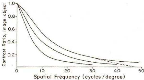
FIG. 9. Modulation transfer functions (MTFs) of the human eye for various pupil diameters. Each curve shows contrast reduction (i.e., retinal image contrast divided by the object contrast) imposed on sinusoidal targets as function of their spatial frequency. Solid curves (from top to bottom ) correspond to pupil diameters of 2.4, 3.8, and 6.6 mm; dashed curve corresponds to 1.5 mm. MTFs calculated from linespread data of Fig. 6. [From Gubisch (59).]
