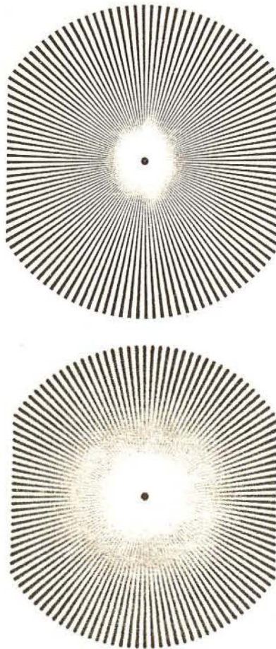
FIG. 11. Top : spoke target for demonstrating spurious resolution in human vision. See text for directions. Bottom : out-of-focus picture of spoke pattern illustrating spurious resolution in a photographic image.
