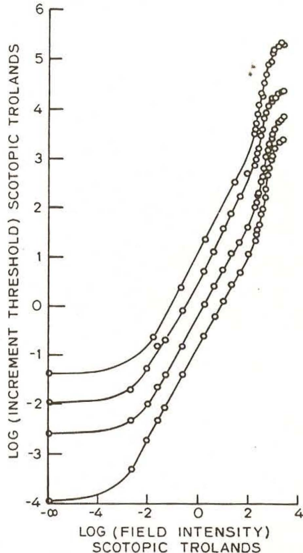
FIG. 32. Increment-threshold curves for rod-initiated detection. Test stimulus, 9^\circ diam, 0.2 s, centered 9^\circ from fovea. Conditioning field, 20^\circ diam, exposed steadily. Means from four observers are shown. Lowest curve correctly placed with respect to both axes. Other curves displaced upwards by 0.5, 1.0, and 1.5 log units, respectively. [From Aguilar and Stiles (1a).]
