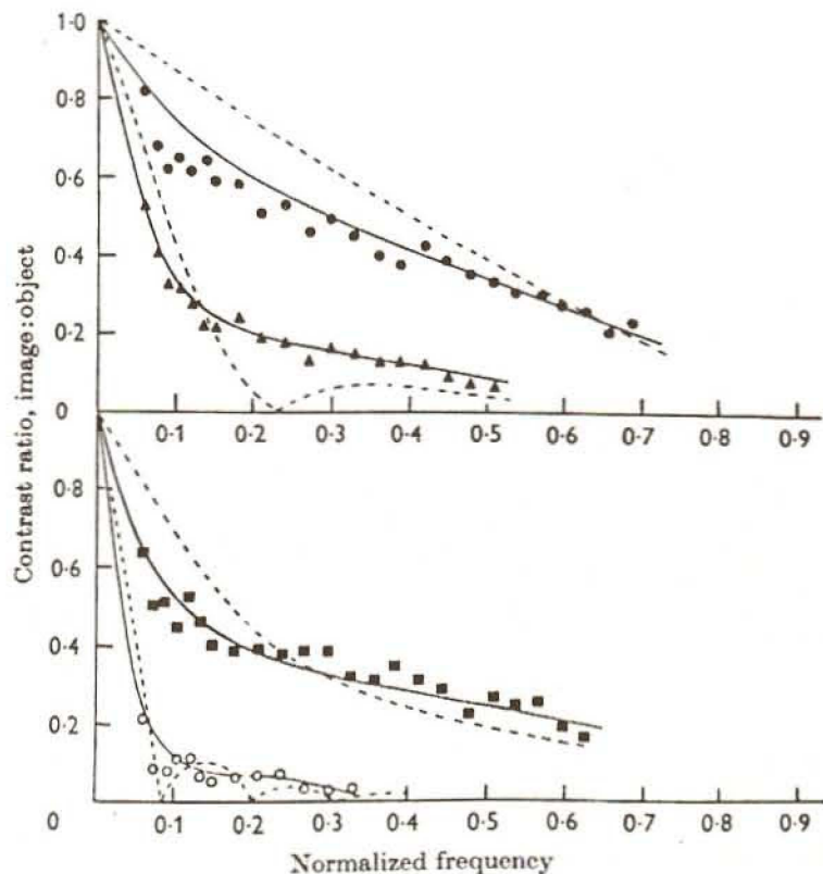
FIG. 10. Effects of defocus on human spatial contrast sensitivity (2-mm pupil). Data points show retinal image contrast reduction (inferred from threshold data of one observer) imposed on each spatial frequency as a function of defocus. Upper panel: ●, 1.5 diopters (myopic); ▲, 2.5 diopters. Lower panel: ■, 2.0 diopters, ○, 3.5 diopters. Spatial frequency expressed as fraction of highest frequency passed by the optics of the eye, i.e., 1.0 \approx 60 cycles/deg. Solid lines drawn by hand through data points. Dashed lines show results predicted from diffraction alone. [From Campbell and Green (32), with permission from Cambridge University Press.]
