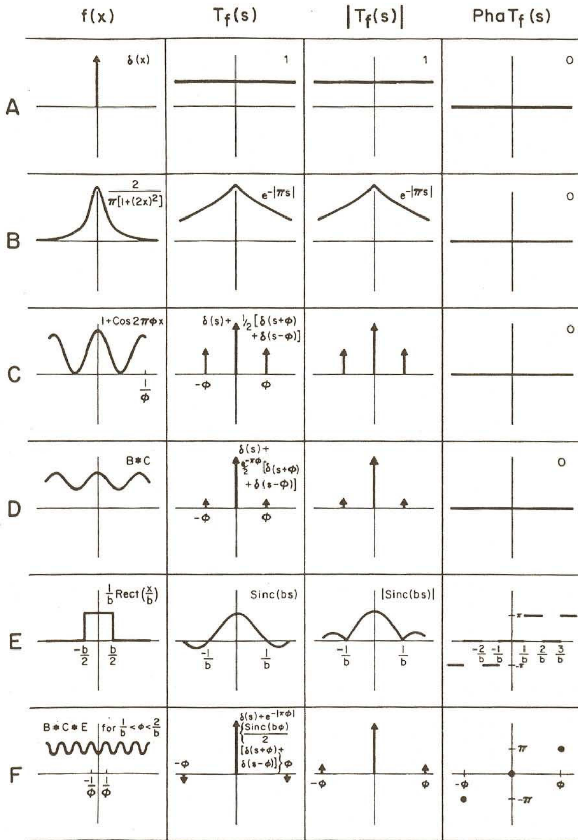
FIG. A1. Fourier analytic concepts involved in one-dimensional spurious resolution. See text for description.
