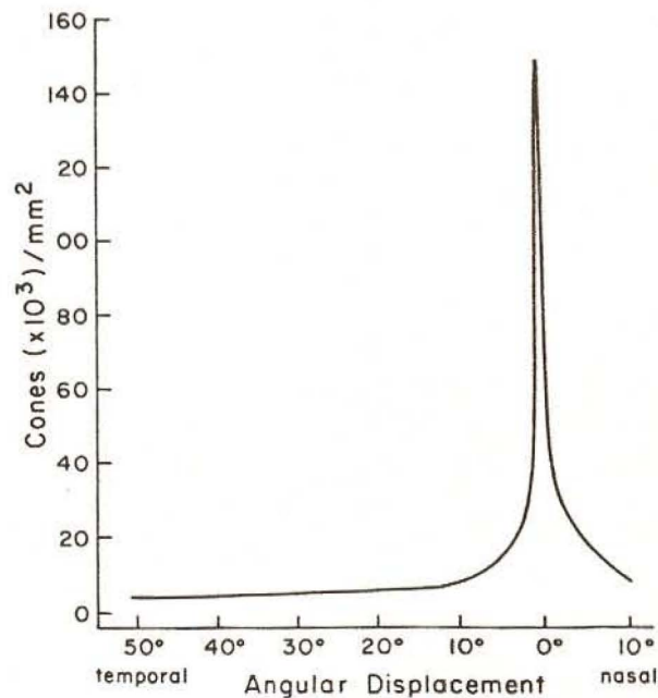
FIG. 13. Cone density as a function of distance from the center ( 0^\circ ) of the fovea. [Data from Osterberg (95); figure adapted from Ripps and Weale (103).]
