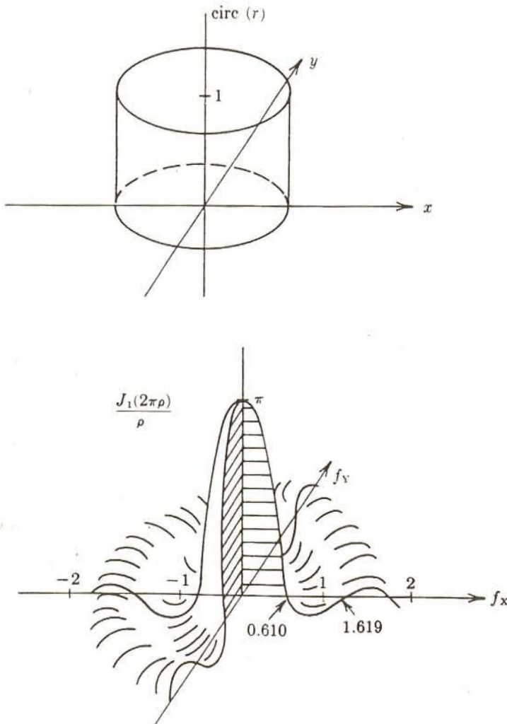
FIG. A2. Two-dimensional disk function (top) and its Fourier transform (bottom). Up to a constant factor \pi , the latter is the graph of Equation A18. [From Goodman (51).]
