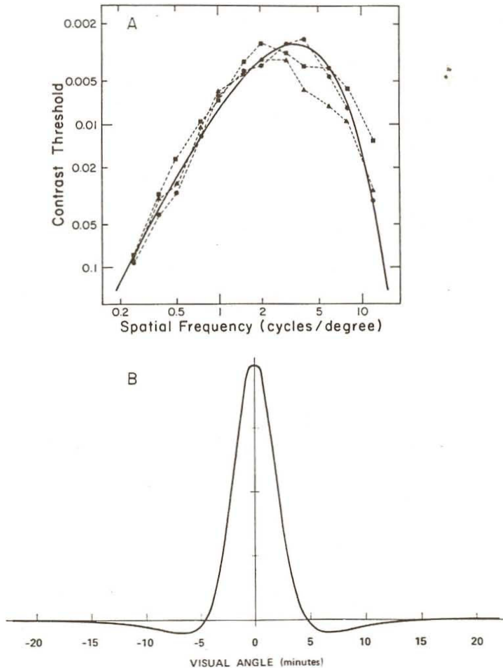
FIG. 17. A: spatial contrast-sensitivity functions for three observers (dashed lines) with fitted function s^2 e^{-s} (solid curve), which can be regarded as the overall "modulation transfer function" of the human visual system. B: pointspread function obtained by Fourier inversion of the smooth curve in Figure 17A. [From Kelly (74).]
