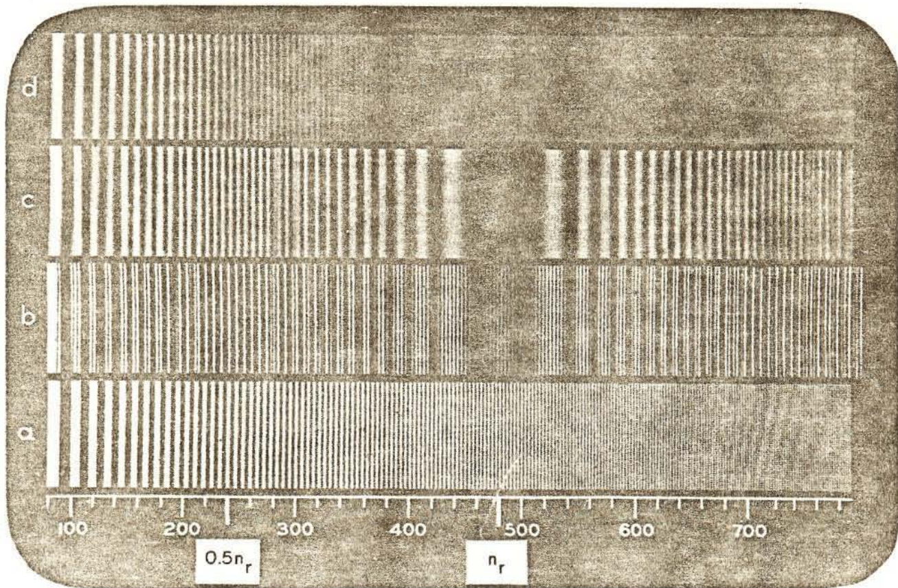
FIG. A4. One-dimensional aliasing effects. Row a is a linearly increasing frequency pattern. Row b shows the sampled appearance of pattern a viewed through a raster plate consisting of fine vertical slits spaced at a frequency equal to n_r on the scale. (This sampling rate guarantees perfect reconstruction for frequencies up to 0.5 n_r , with aliasing distortion for higher frequencies.) Row c shows the effect of spatially postfiltering the sampled image b (in this case by adjusting the scanning spot size in a television camera which views pattern b . The visual analogue would be lateral neural interactions at the receptors or beyond.) Notice that this removes the raster lines but does not eliminate aliasing: Frequencies higher than 0.5 n_r still appear as lower frequencies. Row d shows the effect of the spatial postfilter alone (i.e., on pattern a viewed without the raster plate). [From Schade (116).]
