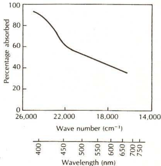
FIG. 20. Absorption spectrum of human ocular media. [From Ludvigh and McCarthy (89).]
