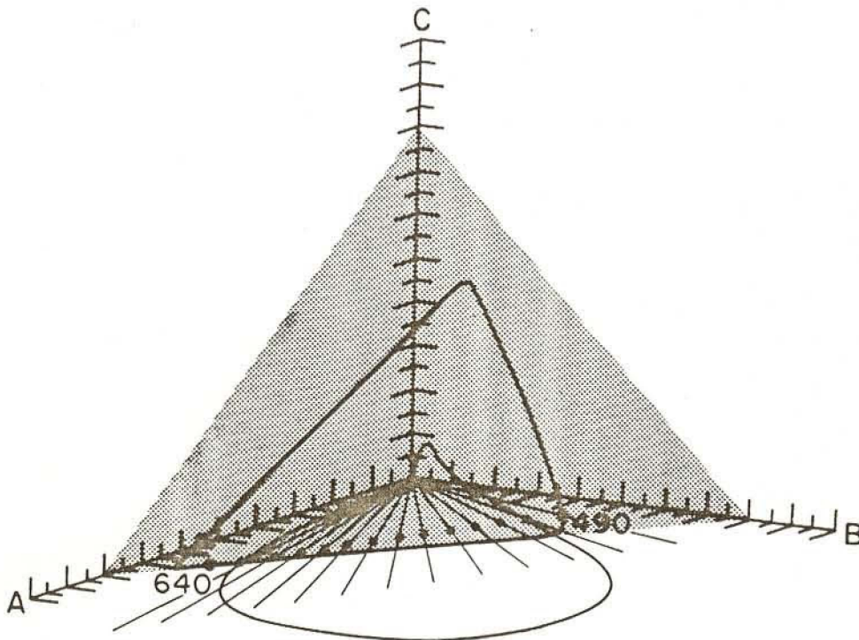
FIG. 30. A representation of the effects of mixtures of lights at 640 nm and 490 nm. As the relative intensities of the two components change, the effect of the mixtures move in a plane indicated by the straight lines emerging from the origin. The intersections of these lines with the shaded plane are indicated by dots, and form a straight line between the points representing 640 nm and 490 nm.
