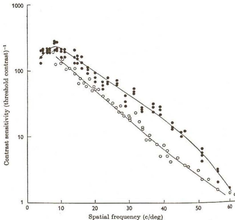
FIG. 14. Spatial contrast-sensitivity functions for sinusoidal interference targets formed with a coherent source; wavelength, 633 nm. Data for two observers; smooth curves drawn by hand through data points. Mean illumination level, 500 trolands. [From Campbell and Green (32), with permission from Cambridge University Press.]
