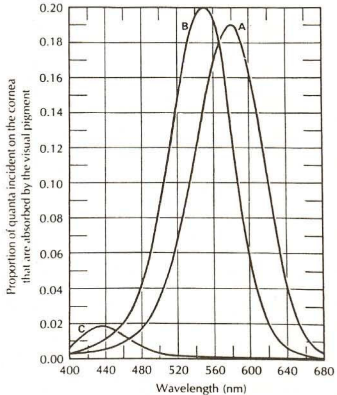
FIG. 27. Estimates of the absorption spectra of the three normal human cone pigments. [From Wald (131). Copyright 1964 by the American Association for the Advancement of Science.]
