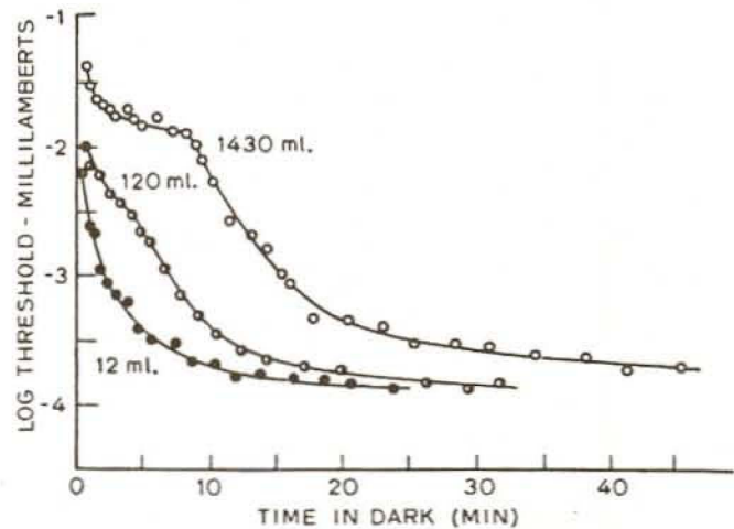
FIG. 35. Dark-adaptation curves following adaptation to conditioning fields of various intensities. [From Winsor and Clark (143).]
