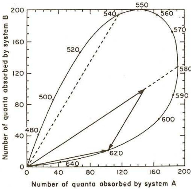
FIG. 26. If a mixture of two wavelengths is to match a third whose effects do not lie on a line between the two to be mixed, one of the two components of the mixture must have a negative intensity, as shown by the downward direction of the 500-nm vector. The physical realization of this negative vector requires the addition of 500 nm light of that magnitude to the 620-nm component.
