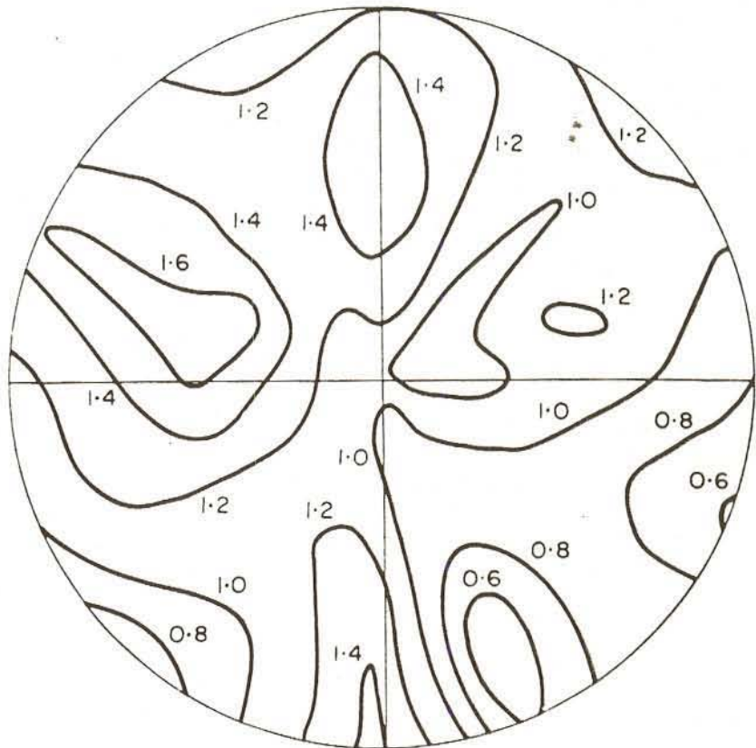
FIG. 3. Irregularities in refractive power across the pupil of a normal eye during relaxed accommodation (pupil diam, 7.2 mm). Contours join points of equal excess power (diopters). [From van den Brink (29a), with permission from Pergamon Press, Ltd.]
