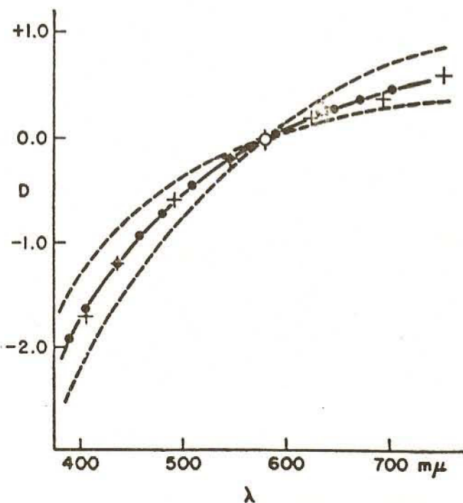
FIG. 2. Chromatic aberration of the human eye. \lambda , Wavelength; D, magnitude of chromatic aberration in diopters (assuming the eye is in perfect focus for 578 nm, D gives the power of the spectacle lens required to focus other wavelengths). Solid line and solid dots, average from 12 observers of Bedford and Wyszecki (19); crosses, average from 14 observers of Wald and Griffin (133); dashed lines, total range for all observations of Bedford and Wyszecki. [Adapted from Bedford and Wyszecki (19).]
