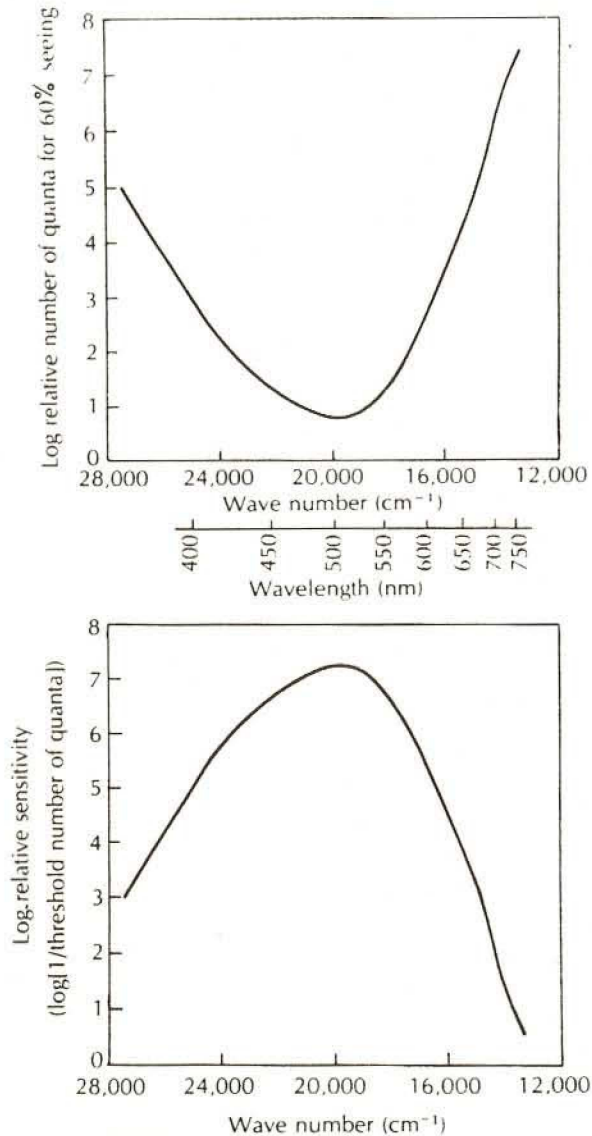
FIG. 19. The scotopic visual action spectrum plotted two ways. Horizontal axis is linear with wave number (number of waves per cm). See text for explanation of data collection procedure. [From Cornsweet (36).]
