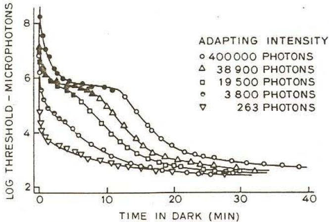
FIG. 33. Dark-adaptation curves follow adaptation to conditioning fields of various intensities. Filled symbols indicate thresholds where the test flash had a colored appearance [From Hecht et al. (65).]
