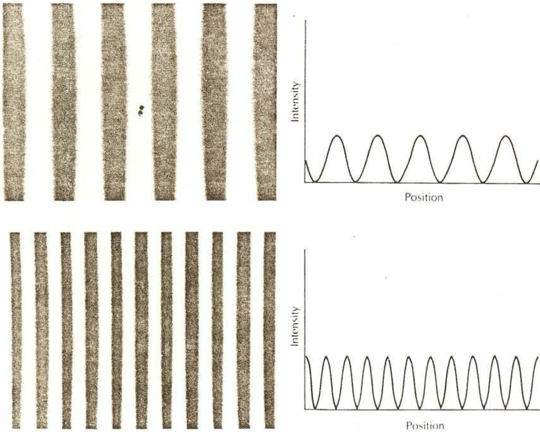
FIG. 8. Sinusoidal gratings. [From Cornsweet (36).]
