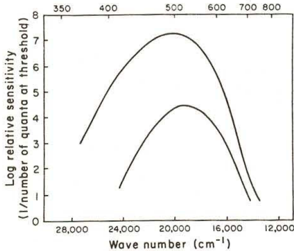
FIG. 22. Spectral sensitivity curve of rods ( upper curve ) compared with spectral sensitivity curve for a hypothetical set of cones ( lower curve ). Note that this lower curve does not represent any real set of cones and is strictly for explanatory purposes.
