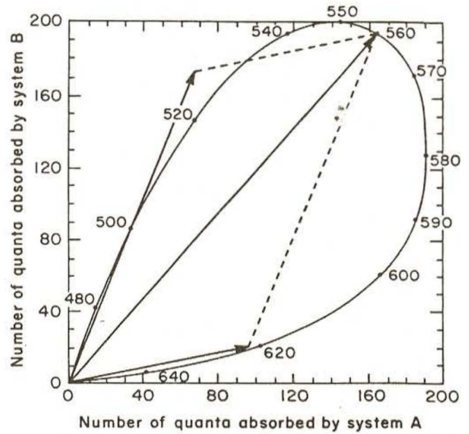
FIG. 25. The effects of a mixture of lights of wavelengths 500 nm and 620 nm and of appropriately chosen intensities (2,050 and 910 quanta·s -1 ·mm -2 , respectively, in this example) will be identical to the effects of a light of 560 nm (at an intensity of 1,000 quanta·s -1 ·mm -2 ).
