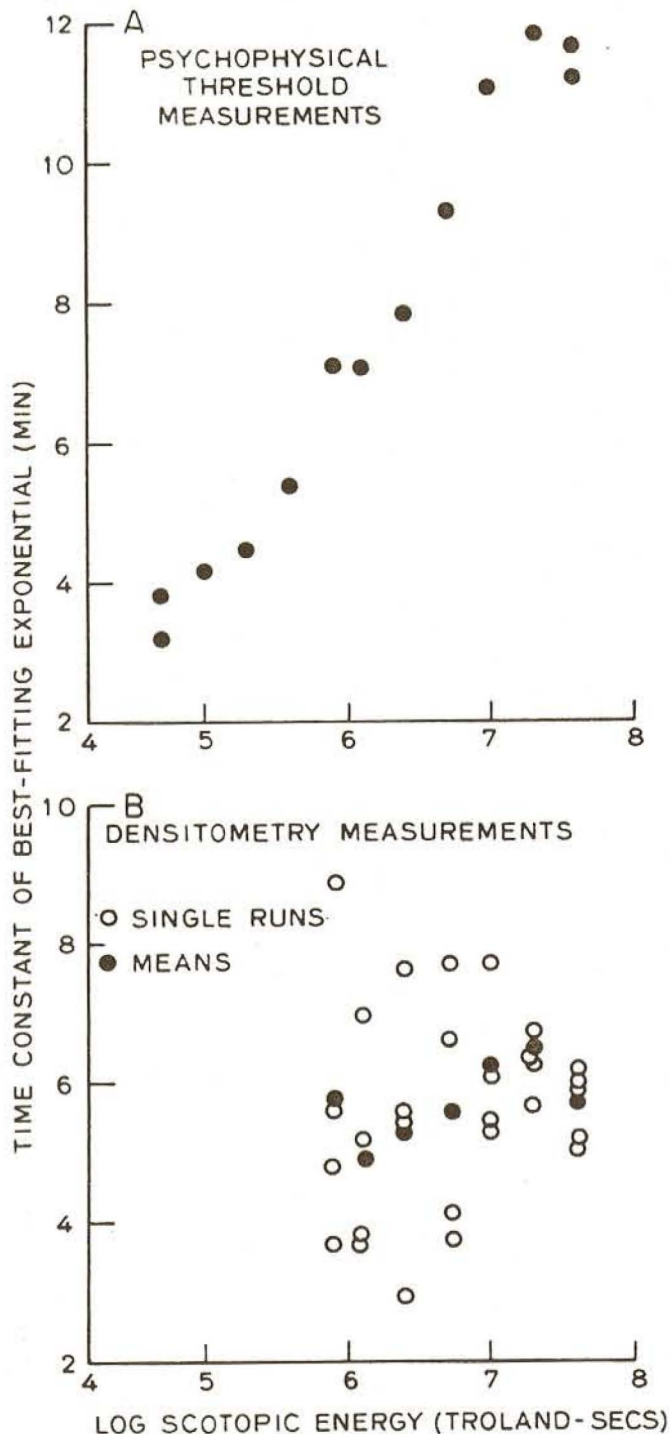
FIG. 36. Time constant of best-fitting exponential curve to A: psychophysical threshold recovery during dark adaptation, and B: rhodopsin regeneration in the living human eye. Both are plotted as a function of energy in the conditioning field. Open symbols in B are individual runs, filled symbols are the arithmetic means of individual runs. [Data from Pugh (100, 101).]
