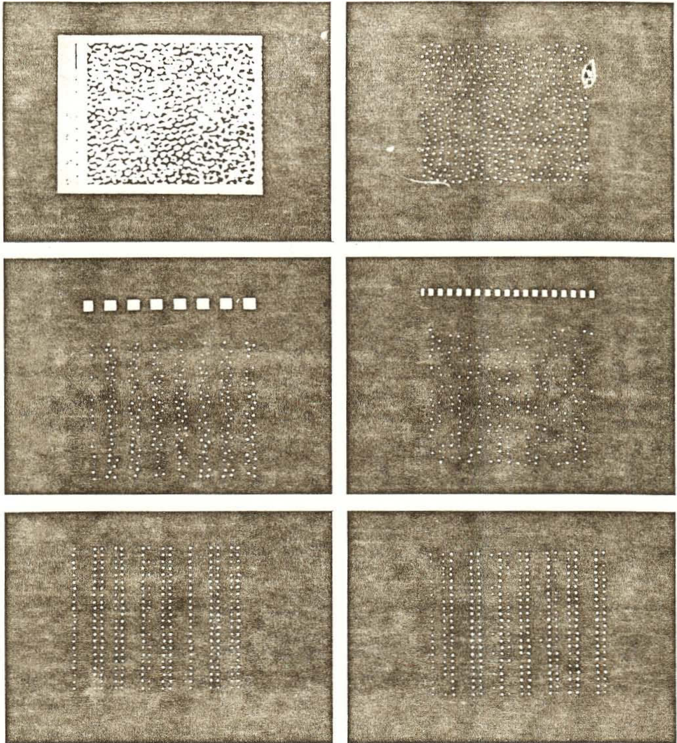
FIG. 18. The top and middle rows illustrate aliasing by an array of photoreceptors. Top left : photomicrograph of a 12' \times 13' patch of human retina near the center of the fovea. The mean center-to-center distance between receptors is 0.53' , implying an aliasing cutoff of 57 cycles/deg. Top right : sampling grid made by punching a pinhole through the center of each receptor in the 12' \times 13' patch. Middle left : 30-cycle/deg square wave grating seen through the pinhole grid. Middle right : 80-cycle/deg square wave grating seen through the pinhole grid. Note the appearance of broad curved line segments due to aliasing. The bottom row illustrates the effect of a regularly spaced (checkerboard) array of sampling points having roughly the same sample-point distance as the average value for the retinal array. Bottom left : 30-cycle/deg square wave grating seen through the regular sampling grid. Bottom right : 80-cycle/deg square wave grating seen through the regular sampling grid. [Top left from Polyak (95), p. 268.]
