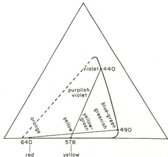
FIG. 31. The hue names of mixtures of 490-nm and 640-nm light change as the ratio of the intensities of the two components change, as indicated along the line between 640 nm and 490 nm. There is a particular mixture of 440-nm and 578-nm lights that will produce an identical hue, as indicated where the two straight lines cross.
