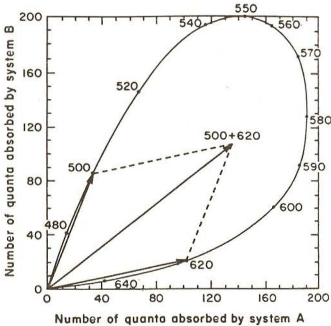
FIG. 24. A representation in two-dimensional action space of the effects of adding lights together. The result can be represented simply as the vector sum of the effects of the components.
