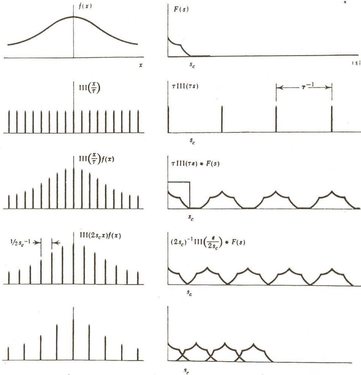
FIG. A3. Concepts involved in the one-dimensional sampling theorem; f(x) is an input signal with transform F(s) which vanishes for s > s_c . \text{III}(x/t) is an infinite row of delta functions (i.e., sample points) spaced t units apart; its transform is a row of delta functions spaced t^{-1} units apart. The third row shows the sampled version of f (i.e., the product f(x) \text{III}(x/t) ) and its transform. Note that here the sampling rate is inefficiently high: successive replicas of F(s) are separated by empty intervals. The fourth row illustrates the optimal sampling scheme, where t = (2s_c)^{-1} : Here the replicas of F(s) in the transform of the sampled signal are precisely adjacent. The fifth row shows the effect of sampling too coarsely: In the transform of the sampled signal the replicas of F(s) overlap (aliasing). [From Bracewell (27). The Fourier Transform and Its Applications (2nd ed.), by R. Bracewell. Copyright © 1978, McGraw-Hill Book Company. Used with permission of McGraw-Hill Book Company.]
