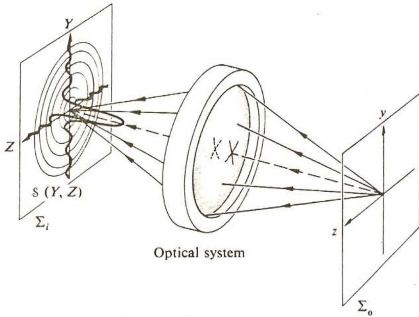
FIG. 4. Pointspread function of an optical system. \Sigma_0 is the object plane, with coordinates y, z ; \Sigma_i is the image plane; S(y, z) , irradiance distribution produced in \Sigma_i by point source located at origin of \Sigma_0 . Illustration is schematic. [From Hecht and Zajac (62).]
