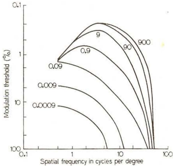
FIG. 12. Human spatial contrast thresholds for vertical sinusoidal gratings at various mean intensity levels (2-mm pupil, monochromatic light, wavelength 525 nm). Each curve plots threshold contrast as a function of spatial frequency for mean retinal illumination level (trolands) indicated by curve parameter (100% corresponds to contrast of 1.0). [Data from Van Ness and Bouman (126); figure from Westheimer (140).]
