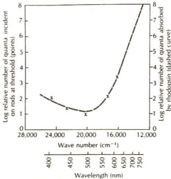
FIG. 21. Scotopic visual action spectrum corrected for absorption by ocular media (x) compared with absorption of rhodopsin (dashed curve). [From Cornsweet (36).]
